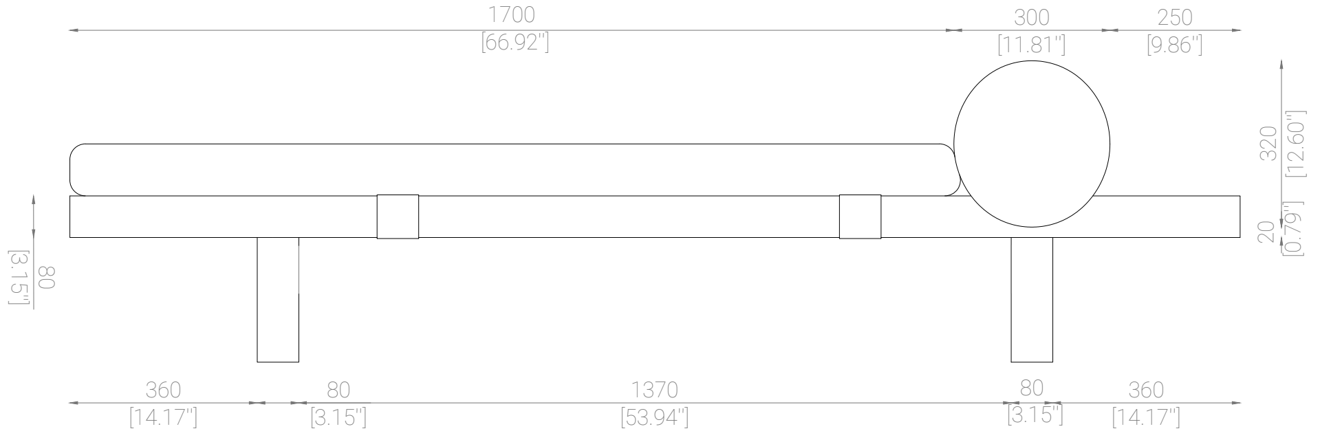
Side Elevation
